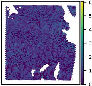
SNU51A THOC7 expression Moran's I = 0.05
