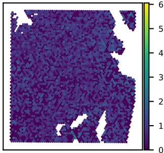
SNU51A NDUFA10 expression Moran's I = 0.02
