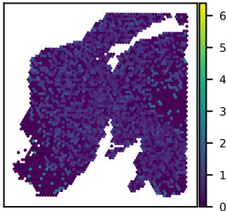
SNU24A C16orf70 expression Moran's I = 0.04
