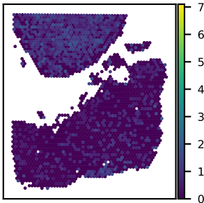
SNU25A CNTNAP2 expression Moran's I = 0.30
