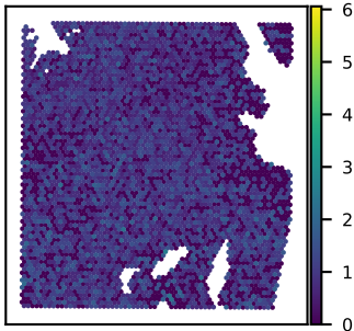
SNU51A SLC25A13 expression Moran's I = 0.06
