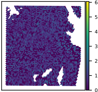
SNU51A RILPL1 expression Moran's I = 0.01
