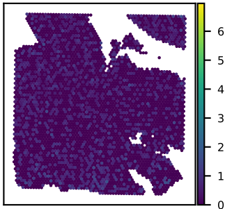
SNU24B MFHAS1 expression Moran's I = 0.01
