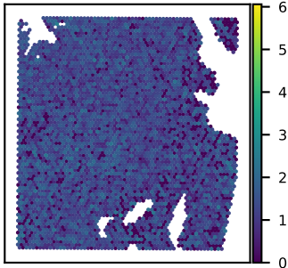
SNU51A SH3GLB1 expression Moran's I = 0.07
