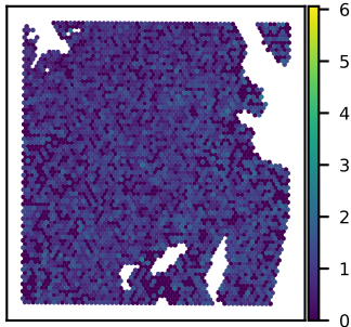
SNU51A SRGAP3 expression Moran's I = 0.03
