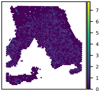
SNU18A CALCRL expression Moran's I = 0.10
