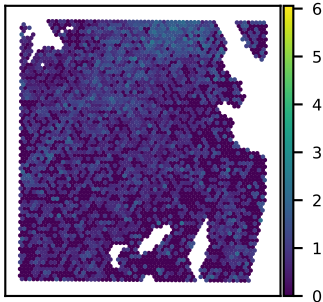
SNU51A PPP1R14A expression Moran's I = 0.20
