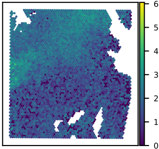
SNU51A SERPINA3 expression Moran's I = 0.50
