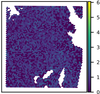
SNU51A BTG2 expression Moran's I = 0.04
