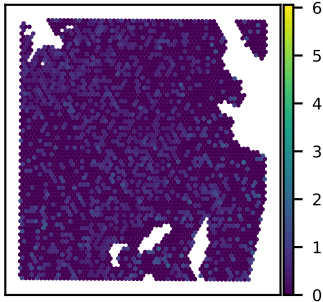
SNU51A SLC26A6 expression Moran's I = 0.01
