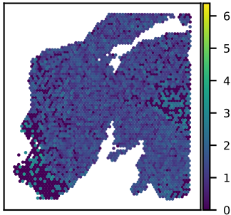
SNU24A POLDIP3 expression Moran's I = 0.05
