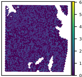
SNU51A GTF3C3 expression Moran's I = 0.00
