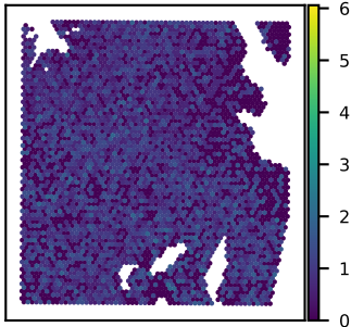
SNU51A VANGL2 expression Moran's I = 0.06
