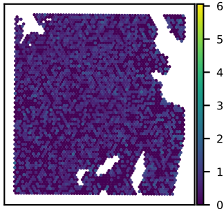
SNU51A DENND11 expression Moran's I = 0.01
