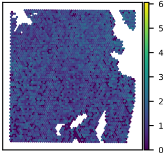
SNU51A MRFAP1L1 expression Moran's I = 0.08
