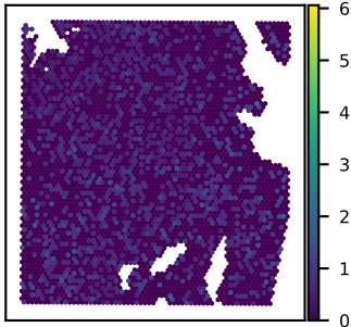
SNU51A CEP97 expression Moran's I = 0.01
