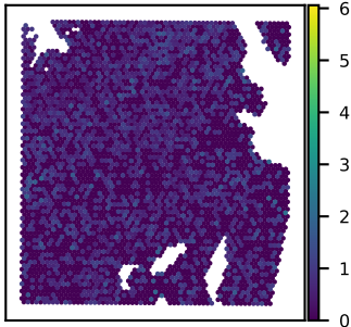
SNU51A MAP3K11 expression Moran's I = 0.03
