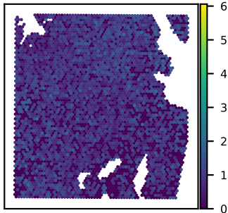
SNU51A PHYHIPL expression Moran's I = 0.06
