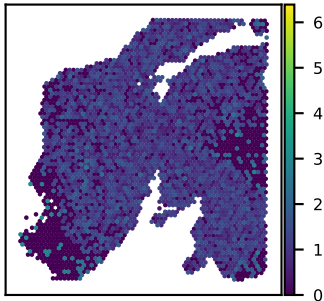
SNU24A TMEM8A expression Moran's I = 0.10
