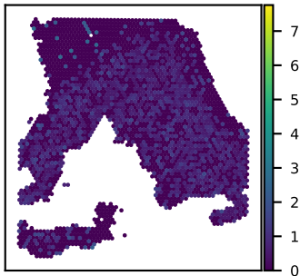
SNU18A SEPTIN6 expression Moran's I = 0.10
