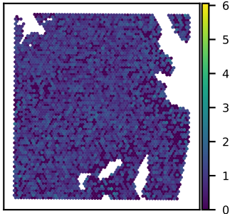
SNU51A TMEM184B expression Moran's I = 0.02
