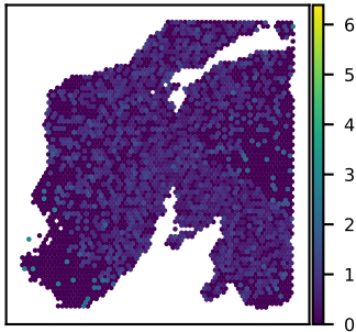
SNU24A SCAMP3 expression Moran's I = 0.06
