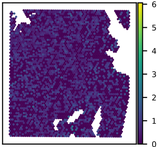
SNU51A ASCC3 expression Moran's I = 0.03
