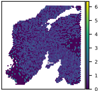
SNU24A MMADHC expression Moran's I = 0.08
