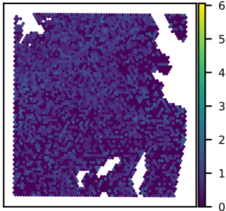
SNU51A ABHD4 expression Moran's I = 0.05
