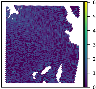
SNU51A LMAN1 expression Moran's I = 0.09
