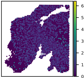
SNU24A C12orf45 expression Moran's I = 0.05
