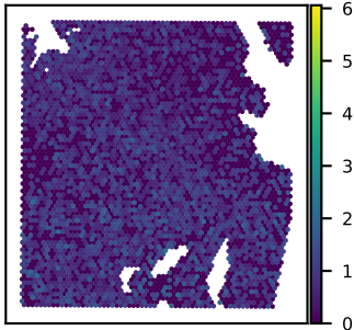
SNU51A NKIRAS2 expression Moran's I = 0.06
