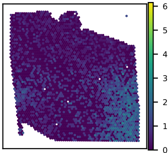
SNU27A C1orf115 expression Moran's I = 0.43
