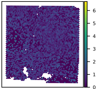
SNU43A MAST4 expression Moran's I = 0.03
