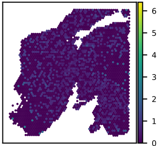
SNU24A ANKRD27 expression Moran's I = 0.03
