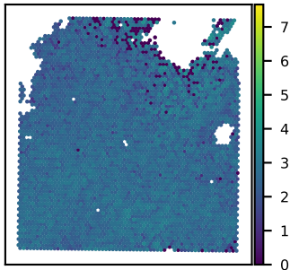
SNU21B CCNI expression Moran's I = 0.16
