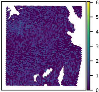
SNU51A ST3GAL4 expression Moran's I = 0.06
