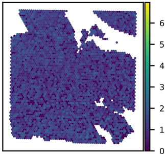
SNU24B DCUN1D4 expression Moran's I = 0.02
