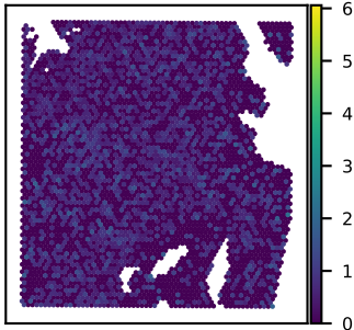
SNU51A PRTFDC1 expression Moran's I = 0.04
