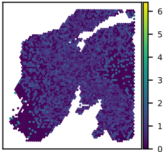
SNU24A AMBRA1 expression Moran's I = 0.06
