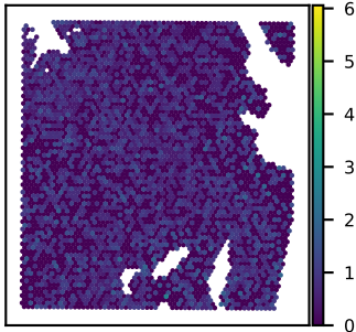
SNU51A NOP58 expression Moran's I = 0.02
