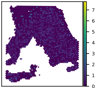
SNU18A GTF3C4 expression Moran's I = 0.03
