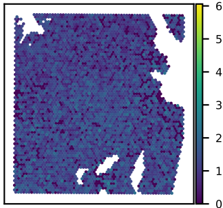
SNU51A BTBD2 expression Moran's I = 0.06
