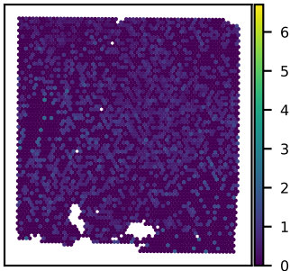
SNU43A C21orf91 expression Moran's I = 0.02
