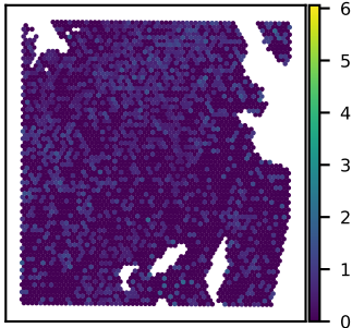
SNU51A HLA-F expression Moran's I = 0.05
