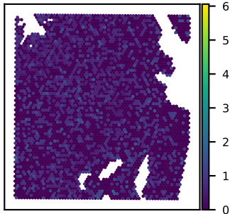
SNU51A ATP8B2 expression Moran's I = 0.02
