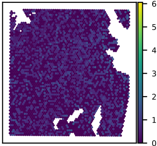
SNU51A BRI3BP expression Moran's I = 0.01
