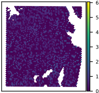
SNU51A CTDP1 expression Moran's I = 0.01
