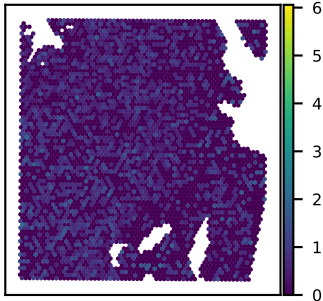
SNU51A ADGRF5 expression Moran's I = 0.04
