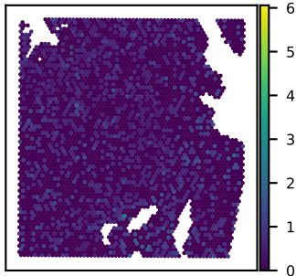
SNU51A KLHL36 expression Moran's I = -0.01
